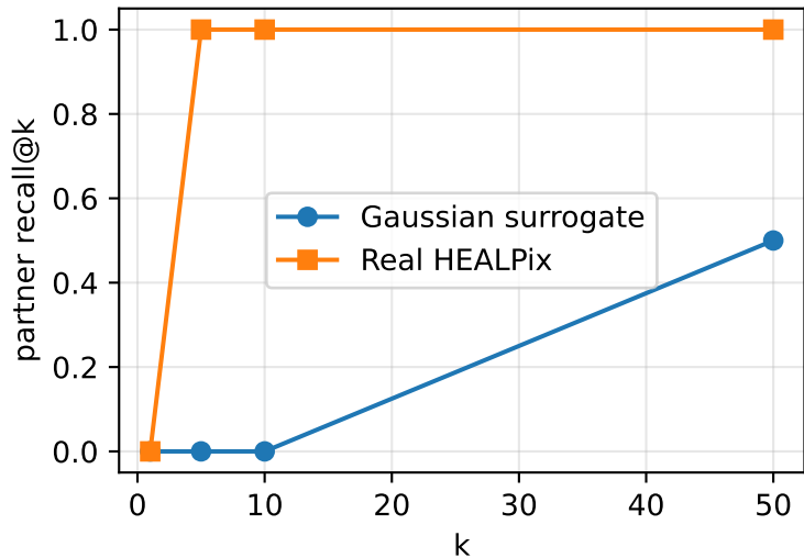
Sky model: surrogate vs real
