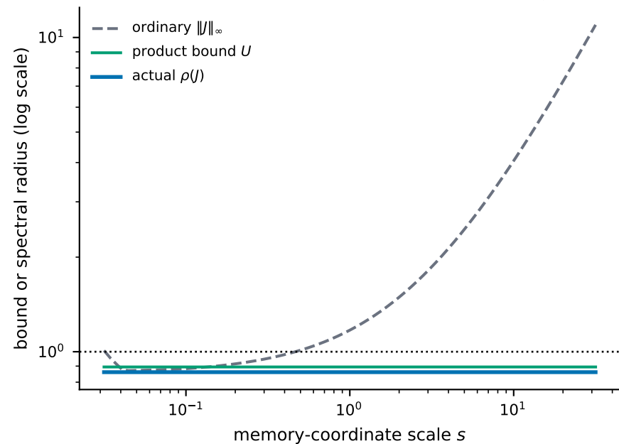
(a) Product bound survives state rescaling
