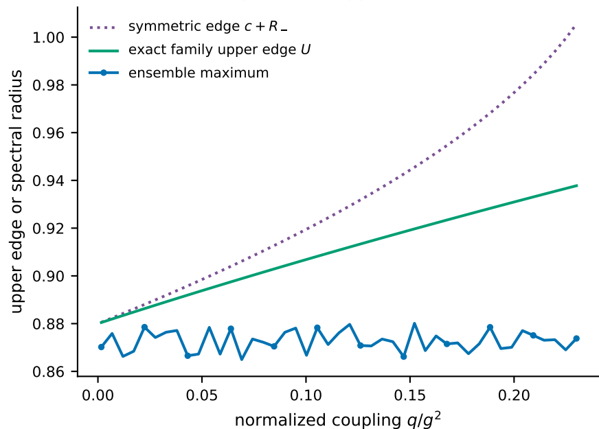
(b) The asymmetric upper edge is tighter
