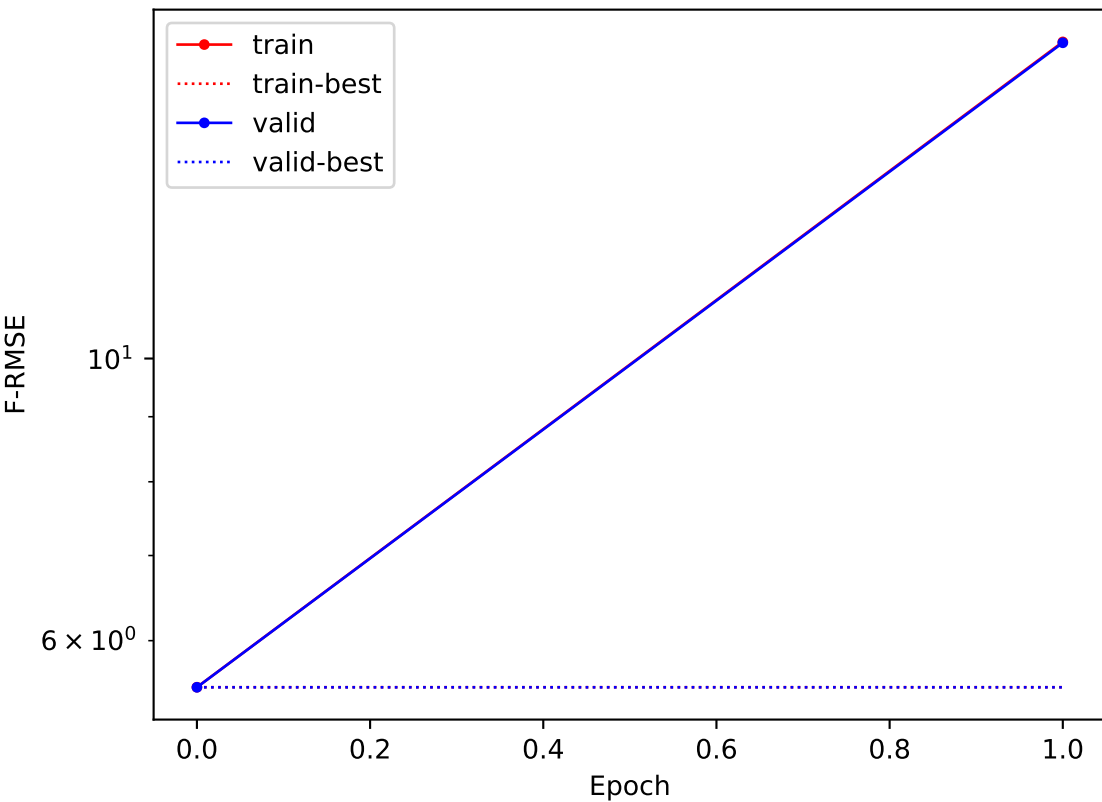
F-RMSE
