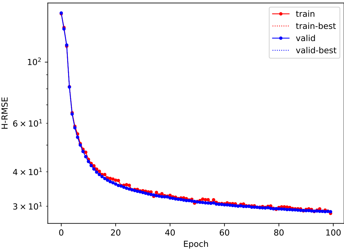
H-RMSE
