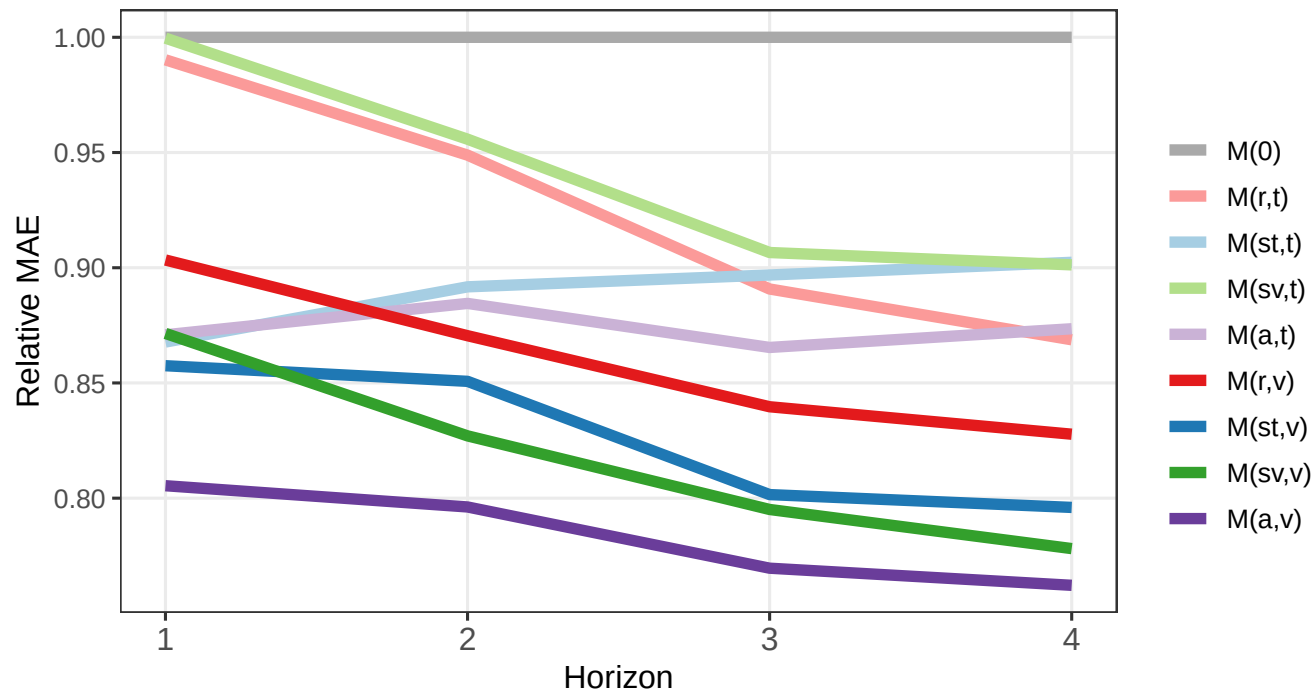
Relative MAE by Model
