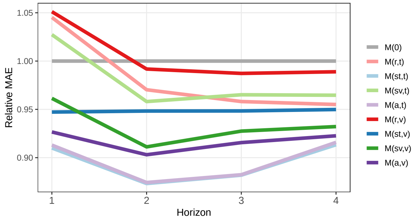
Relative MAE by Model: 2020-07-28 – 2021-12-21
