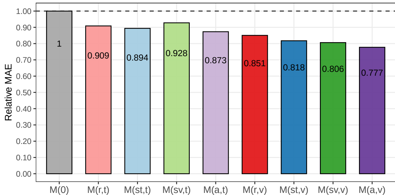
Relative MAE by Model
