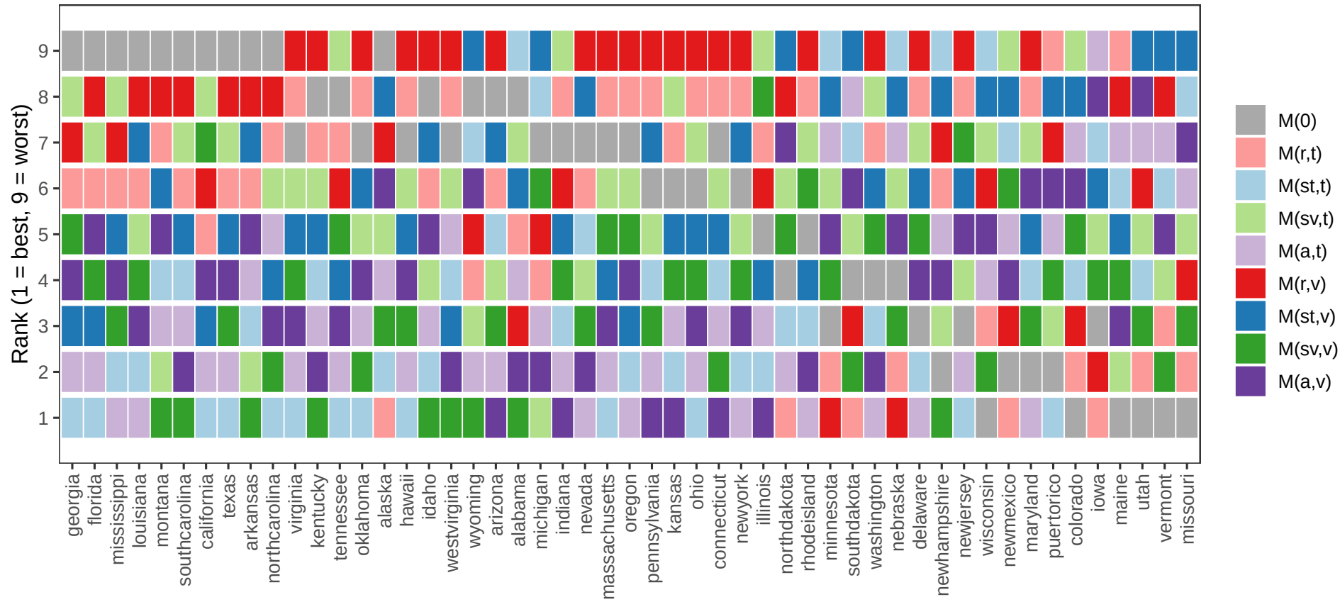
Relative MAE Rank by State: 2020-07-28 – 2021-12-21
