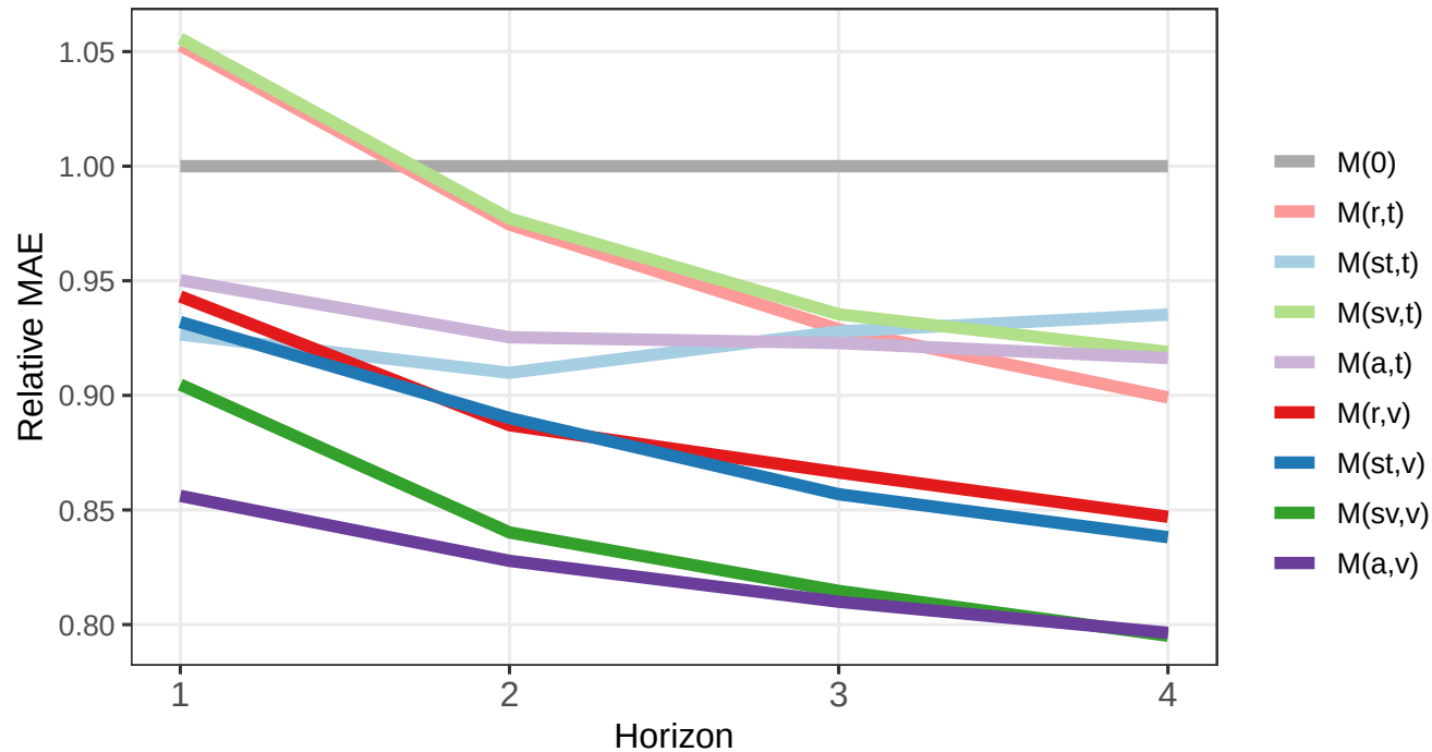
Relative Standardized MAE by Model
