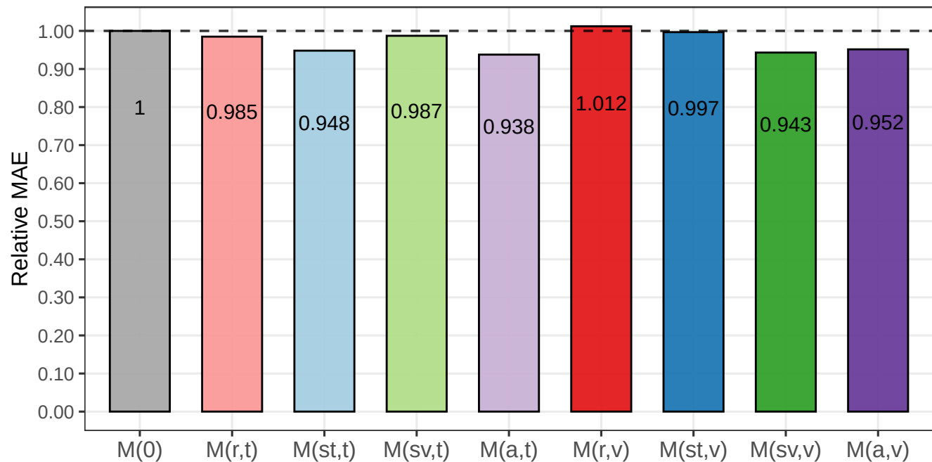
Relative Standardized MAE by Model: 2020-07-28 – 2021-12-21
