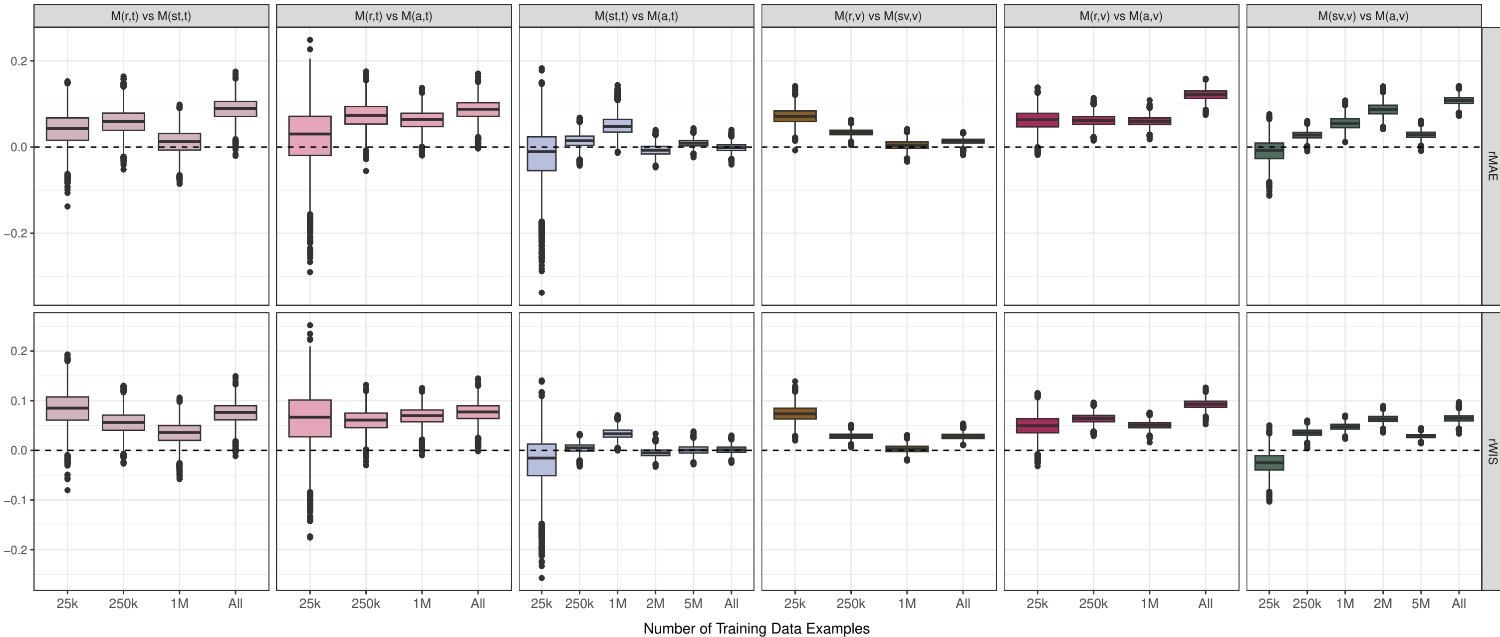
Paired Differences
