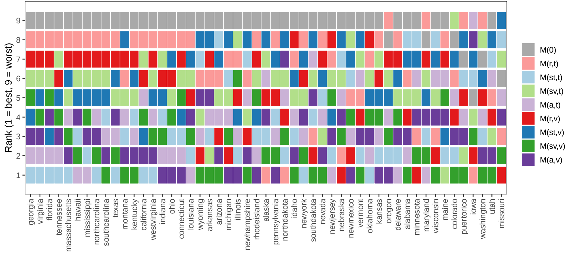
Relative WIS Rank by State: 2020-07-28 – 2021-12-21
