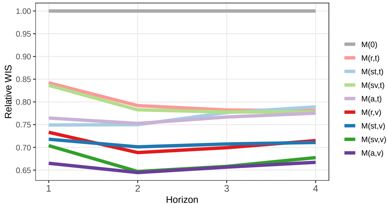
Relative WIS by Model
