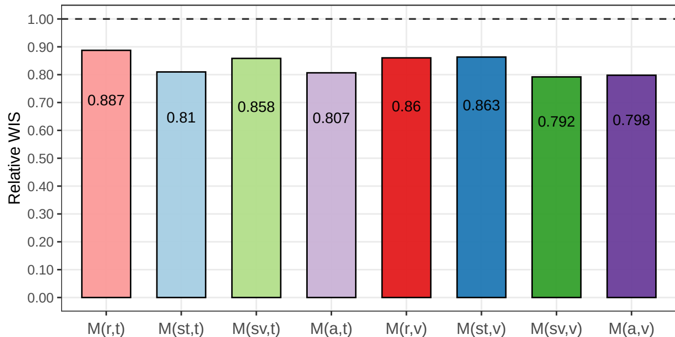
Relative Standardized WIS by Model: 2020-07-28 – 2021-12-21
