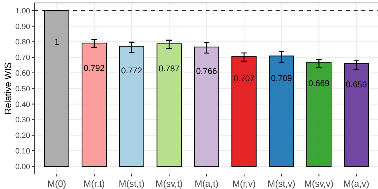
Relative Standardized WIS by Model
