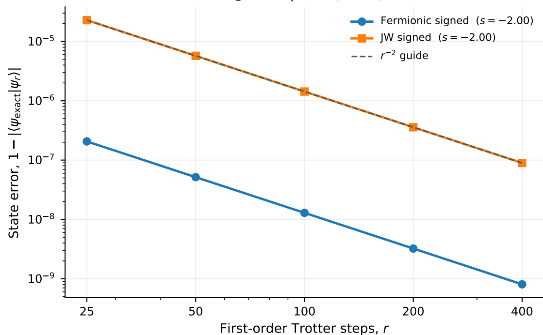
H 2 O: 18 qubits (8+10)
