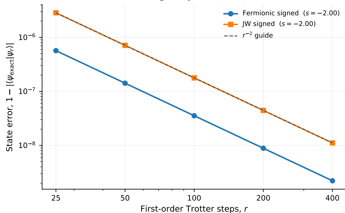
BeH 2 : 18 qubits (6+12)
