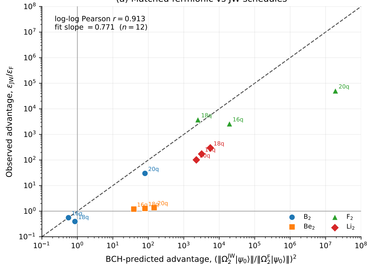
(a) Matched fermionic vs JW schedules
