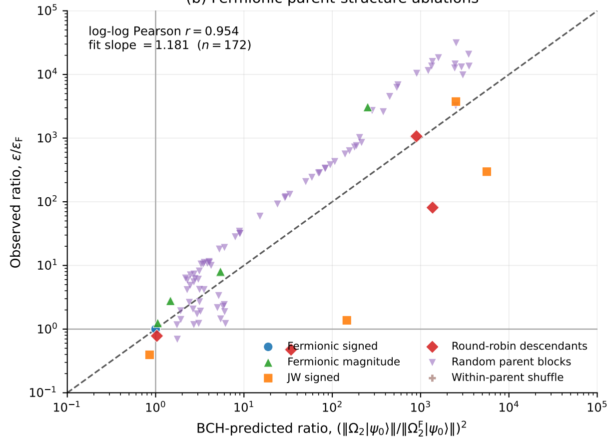
(b) Fermionic parent-structure ablations
