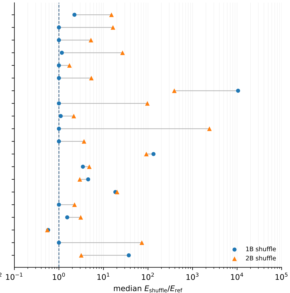
Measured Trotter-error loss
