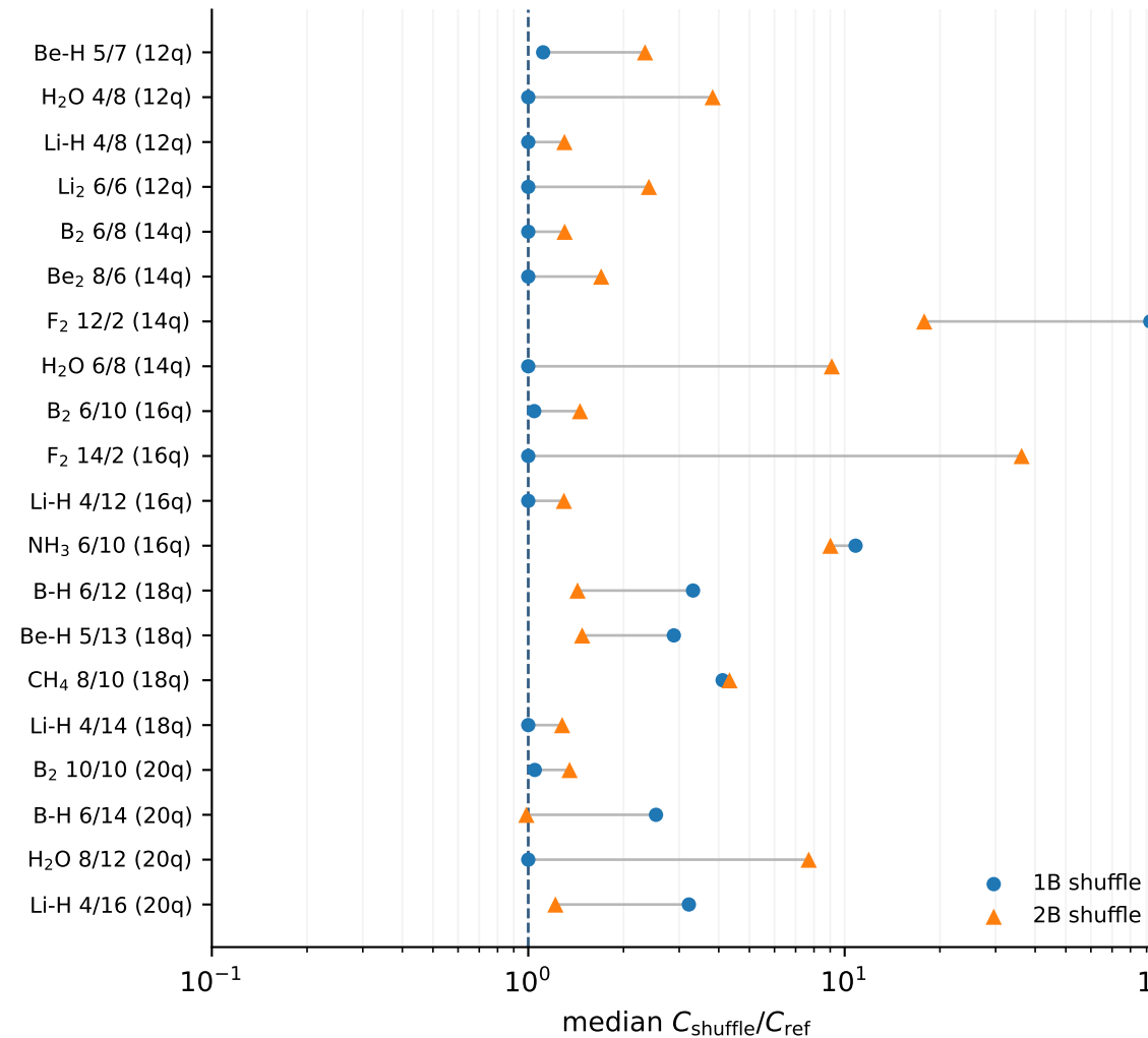
BCH cancellation loss
