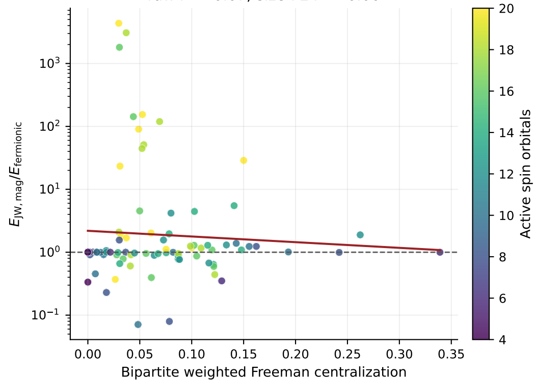
Available HGBS-5 sweep raw r = -0.07 ; size-FE r = -0.06
