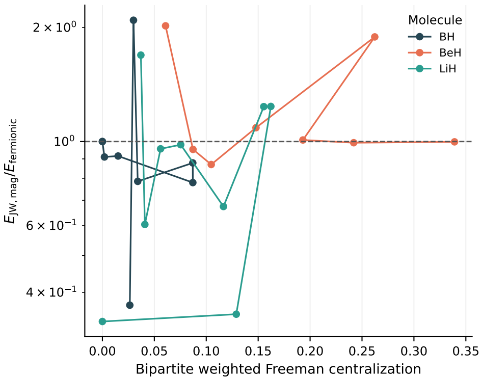
Matched heteronuclear cases raw r = 0.22 ; size-FE r = 0.24
