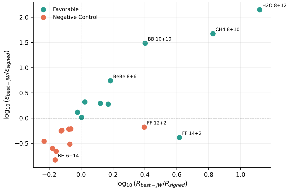
BCH-held-out matched cases
