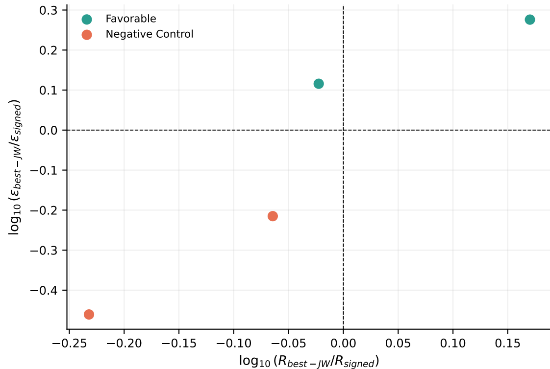
BCH-held-out matched cases
