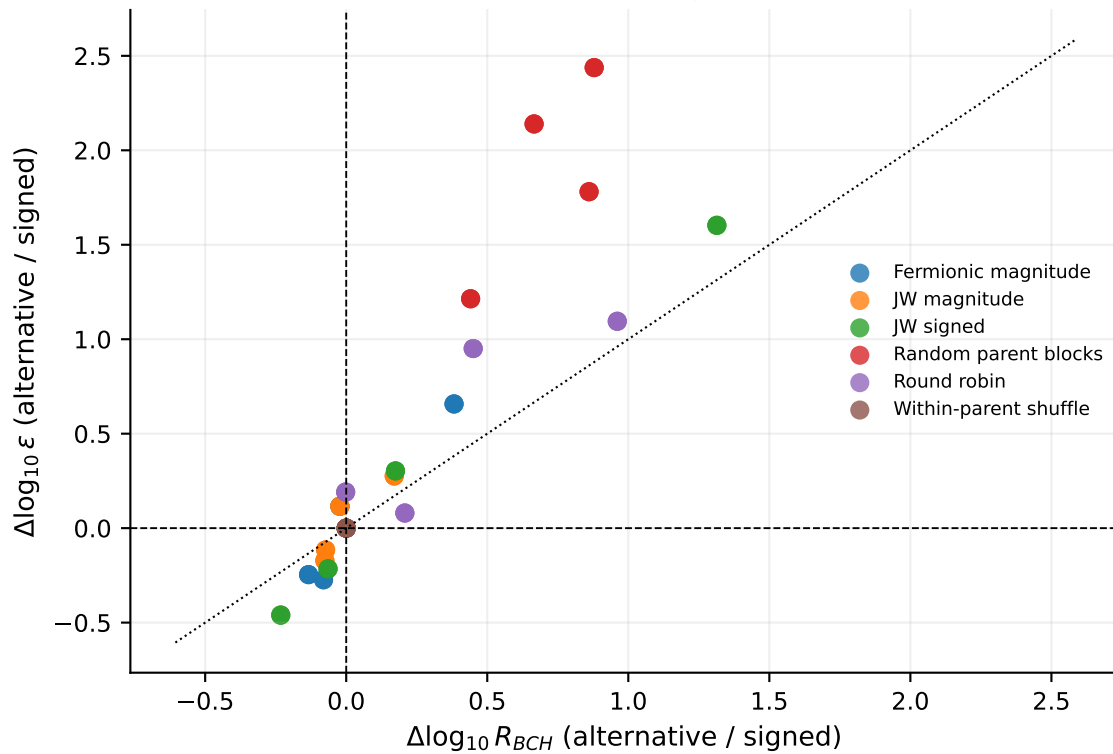
Within-case ordering ablations
