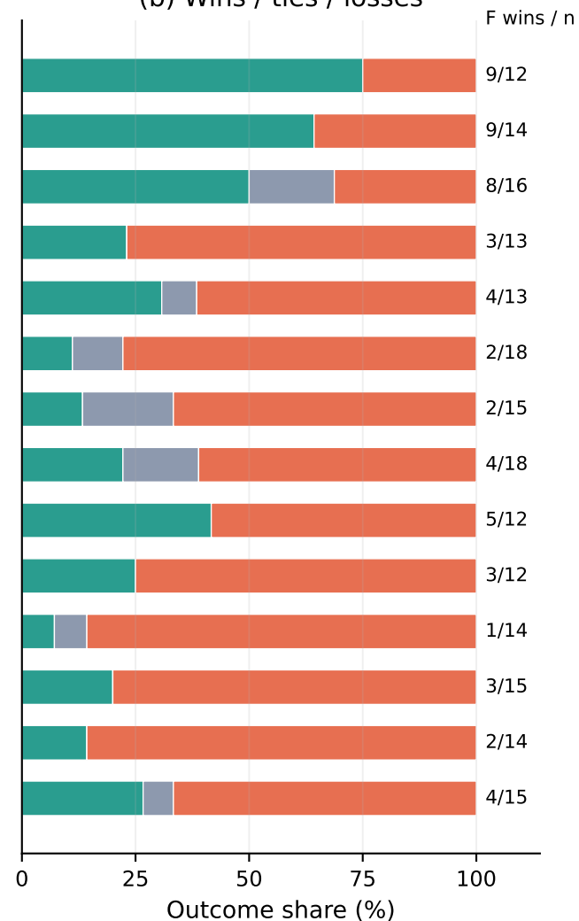
(b) Wins / ties / losses
