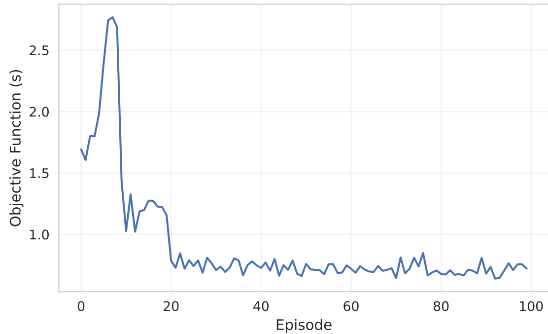
DQN Convergence Analysis
