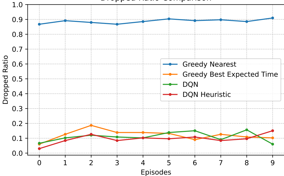
Dropped Ratio Comparison
