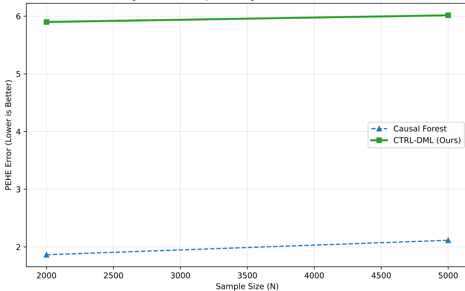
Scaling Law: Can Deep Learning Overtake Trees? (Noise=50)
