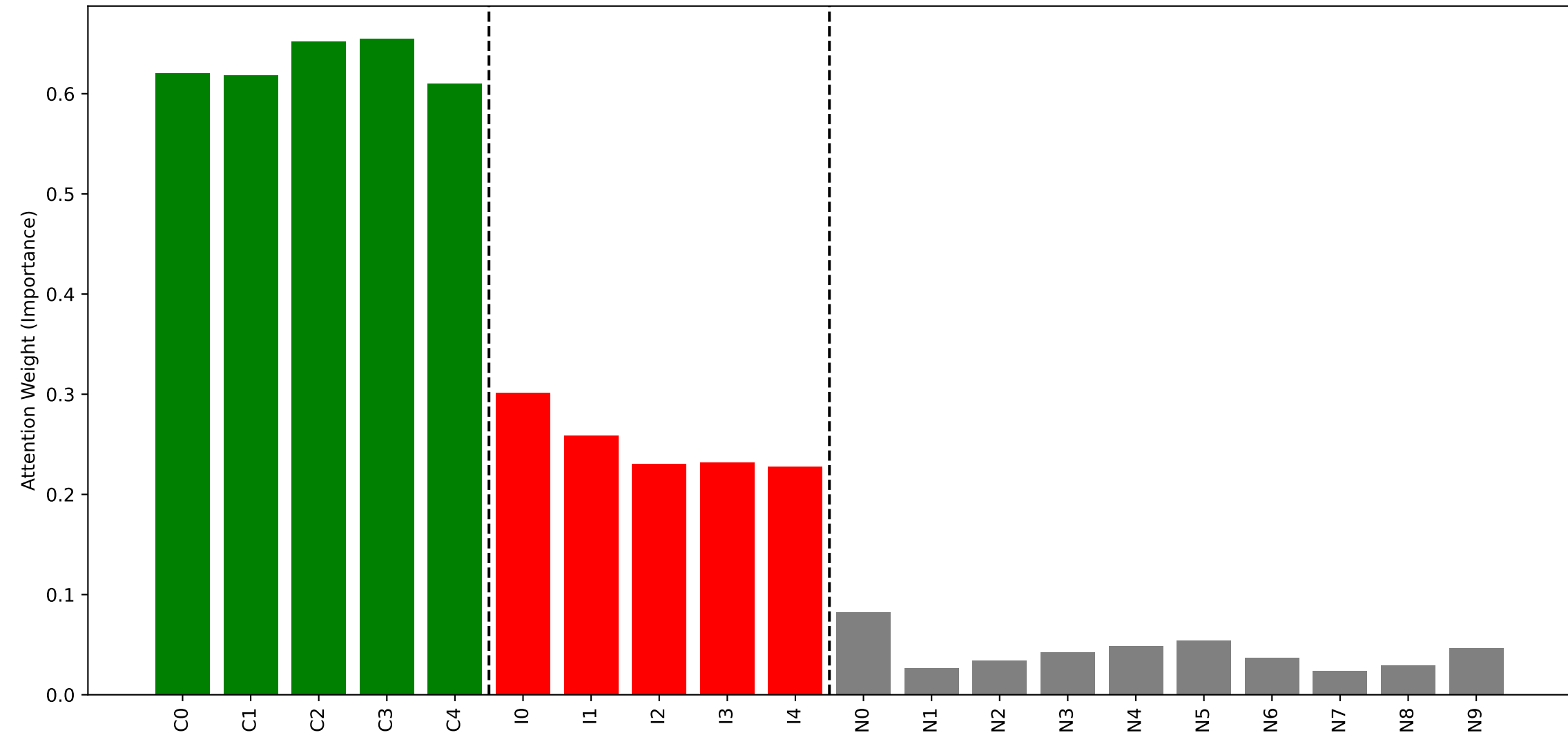
CTRL-DML with Sparsity Penalty ( \lambda=0.05 )
