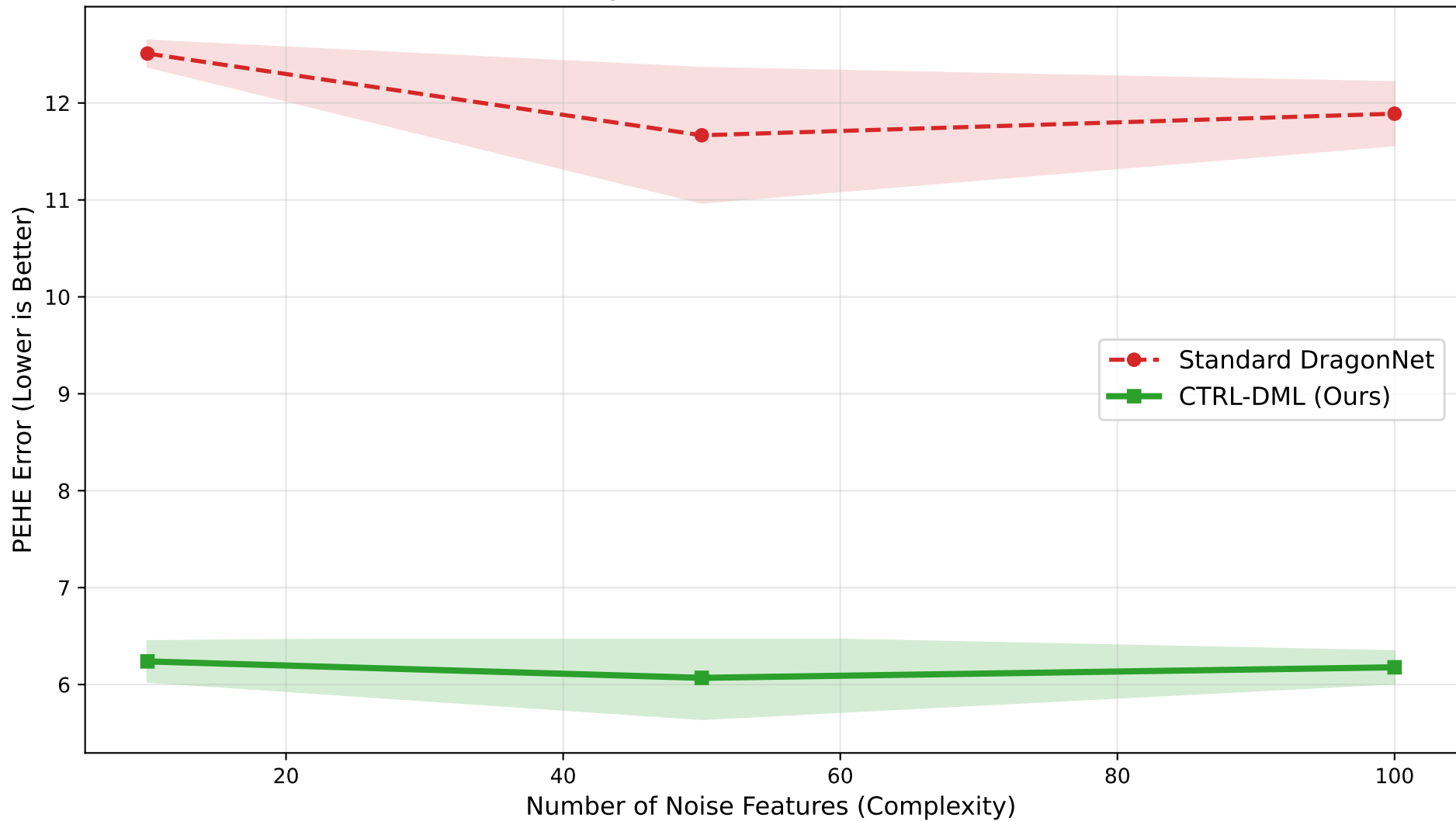
Robustness Analysis with Confidence Intervals (5 Runs)
