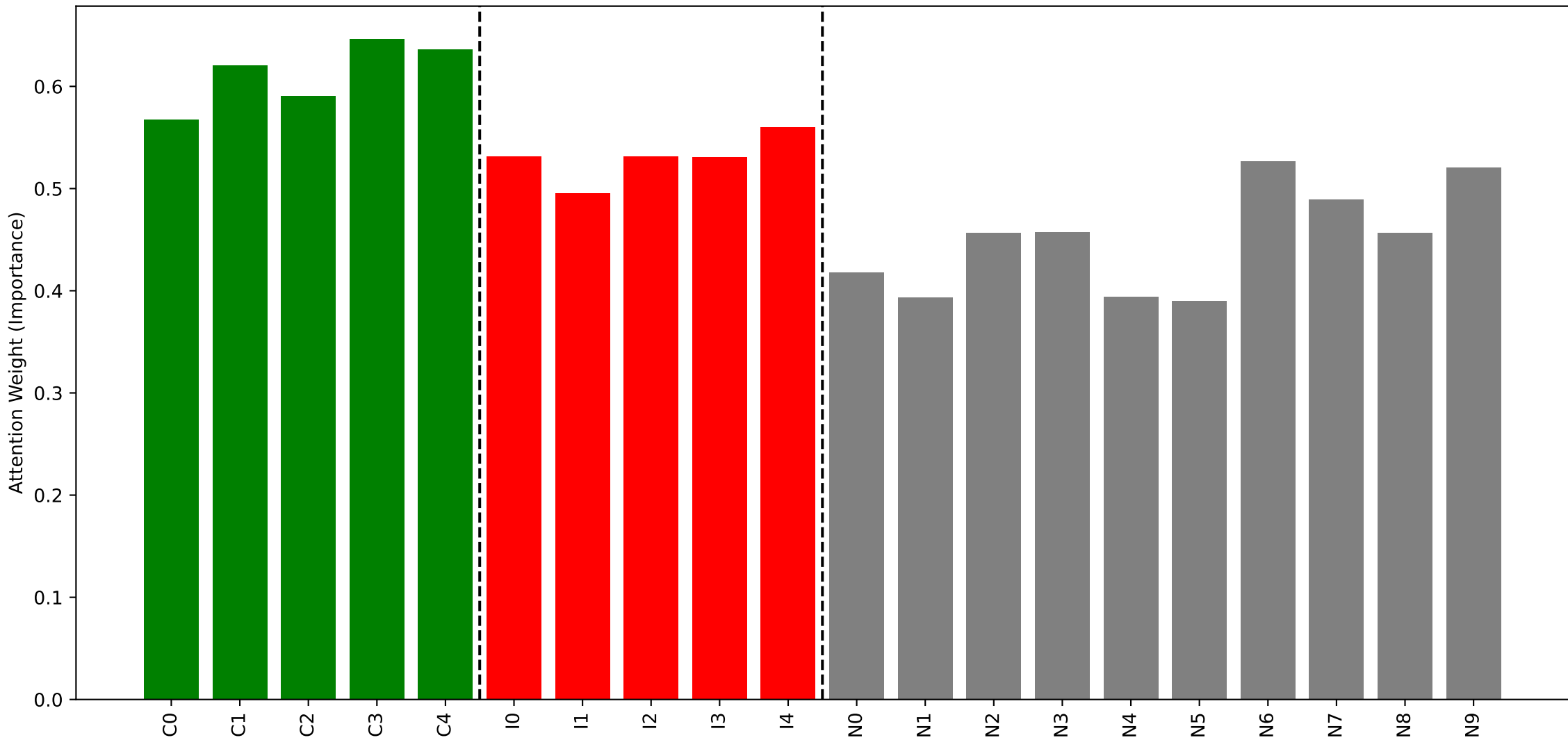
What did CTRL-DML learn? (Green=Confounder, Red=Instrument, Gray=Noise)
