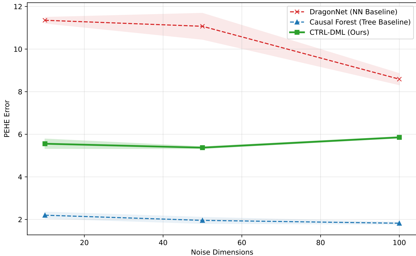
Final Benchmark: Can we beat the Forest?
