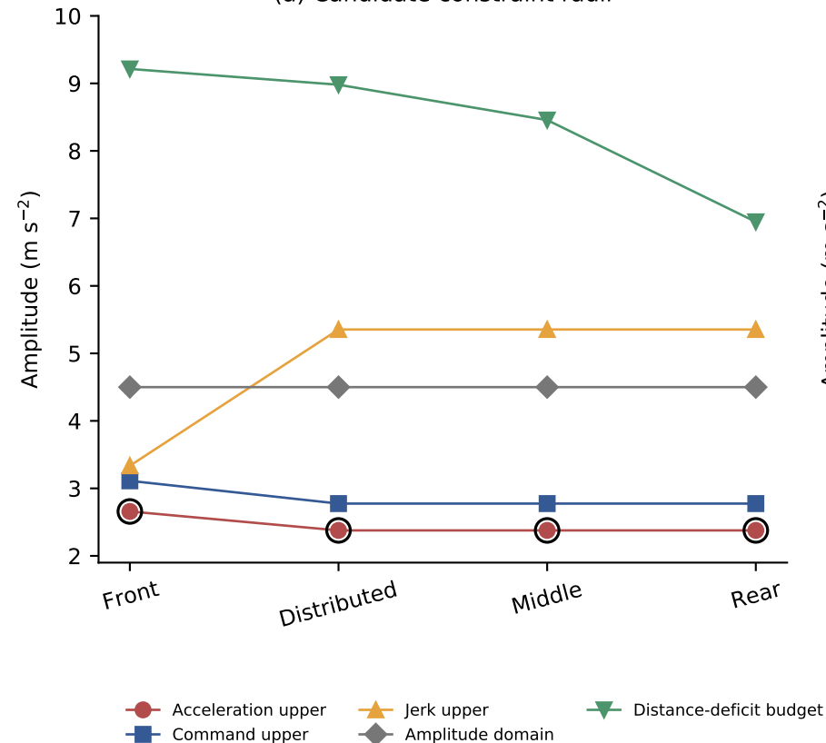
(a) Candidate constraint radii
