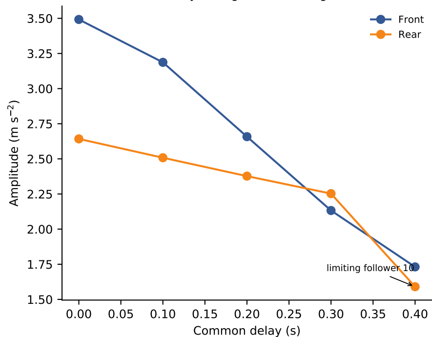
(b) Delay changes the limiting row
