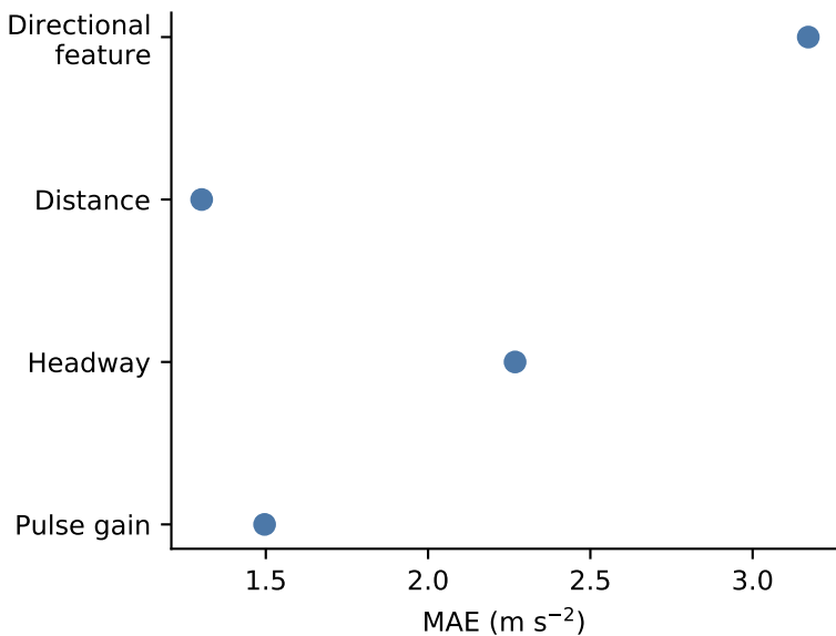
(c) Directional predictor
