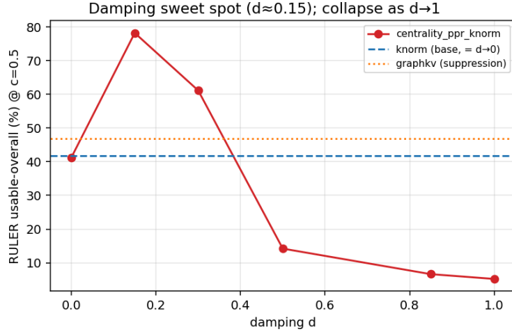
Figure 2: Damping sweep at c=0.5 . A shallow reinforcement ( d \approx 0.15 ) peaks above the base press; as d \rightarrow 1 (pure centrality) it collapses; d \rightarrow 0 recovers the base.
