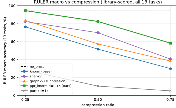
Figure 1: RULER accuracy vs compression
