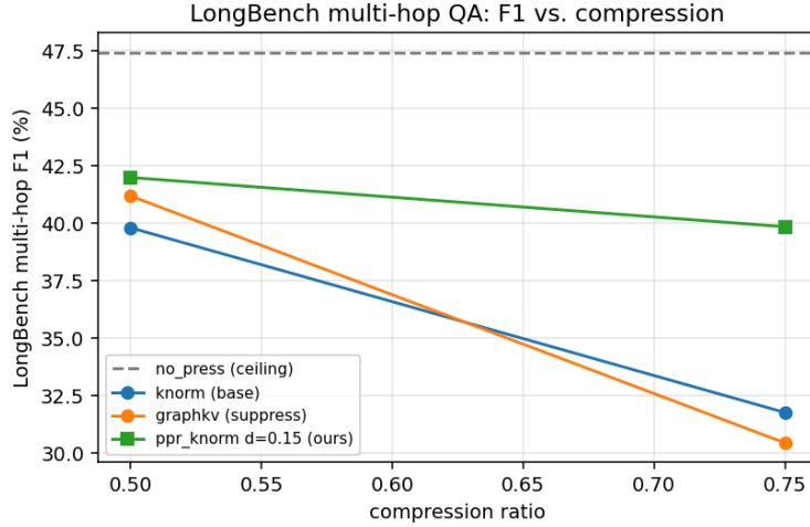
Figure 3: LongBench F1 vs compression
