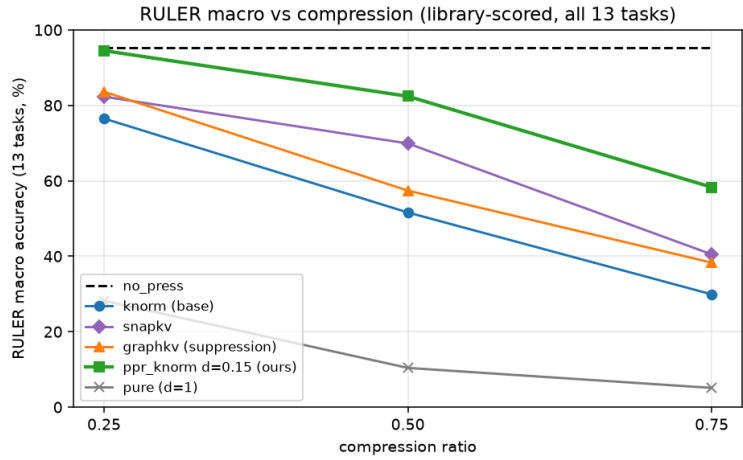
Figure 1: RULER macro accuracy (all 13 tasks, kvpress library scorer, fraction 0.06 screen ) vs. compression. ppr_knorm d=0.15 (ours) dominates its base and the other baselines shown; not a leaderboard-eligible comparison (see cross-method note).
