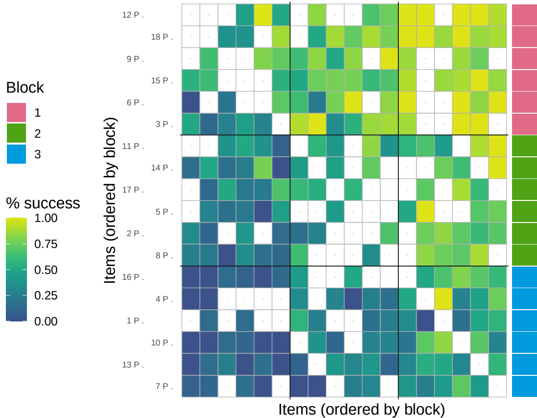
Figure 2: Block-ordered adjacency heatmap. Rows and columns are ordered by inferred blocks, with boundary lines indicating block transitions.
