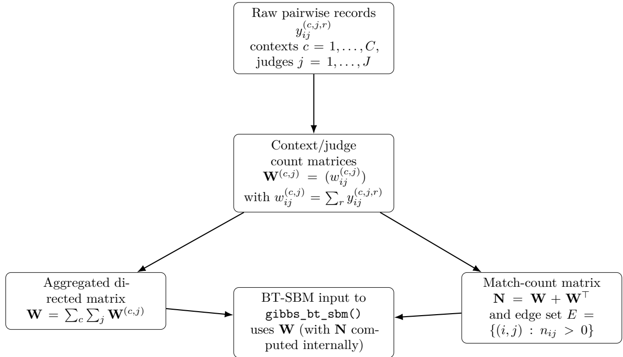
Figure 1: Data-construction map for context/judge pairwise data. Raw comparisons are first summarized into context- and judge-specific count matrices, then aggregated into the adjacency matrix \mathbf{W} used by BT-SBM.
