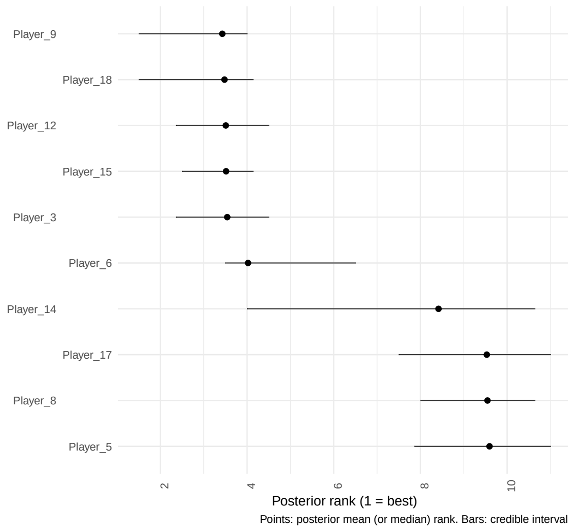
Figure 5: Posterior rank intervals for the top players, highlighting uncertainty in the induced ranking.
