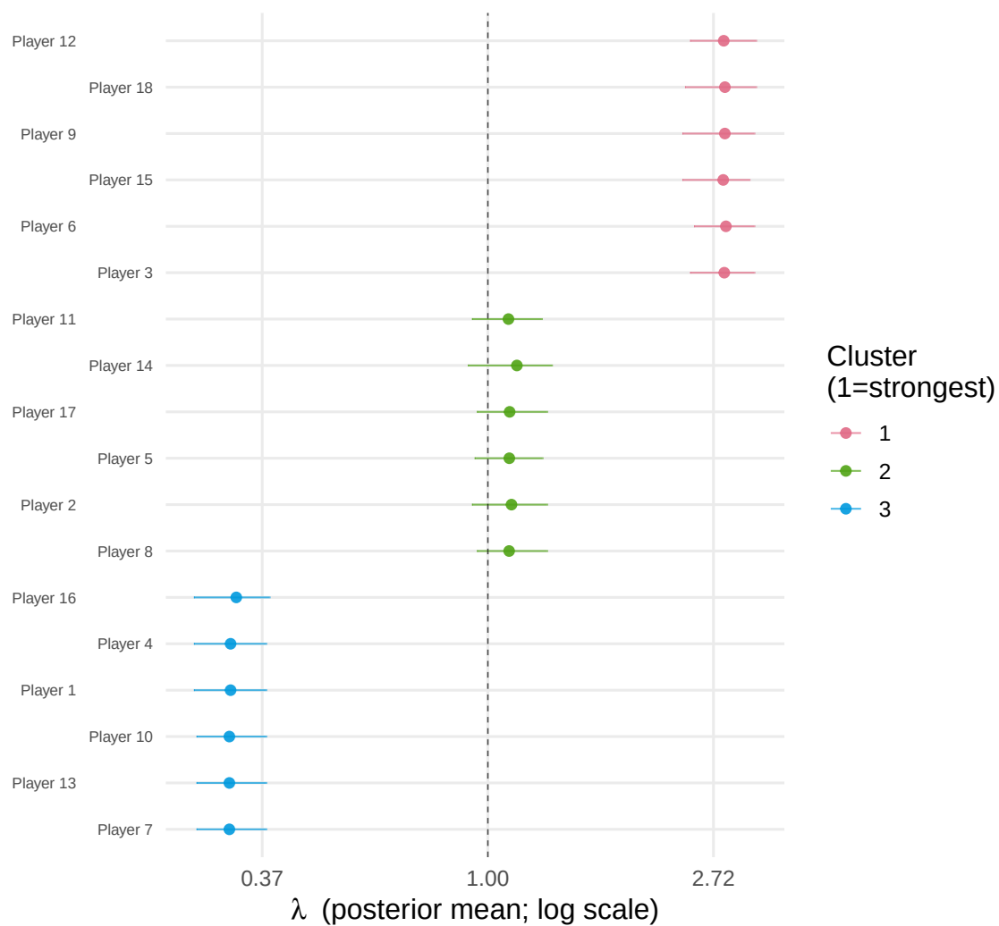
Figure 4: Posterior uncertainty in block intensity parameters (lambda), summarising relative block strengths.
