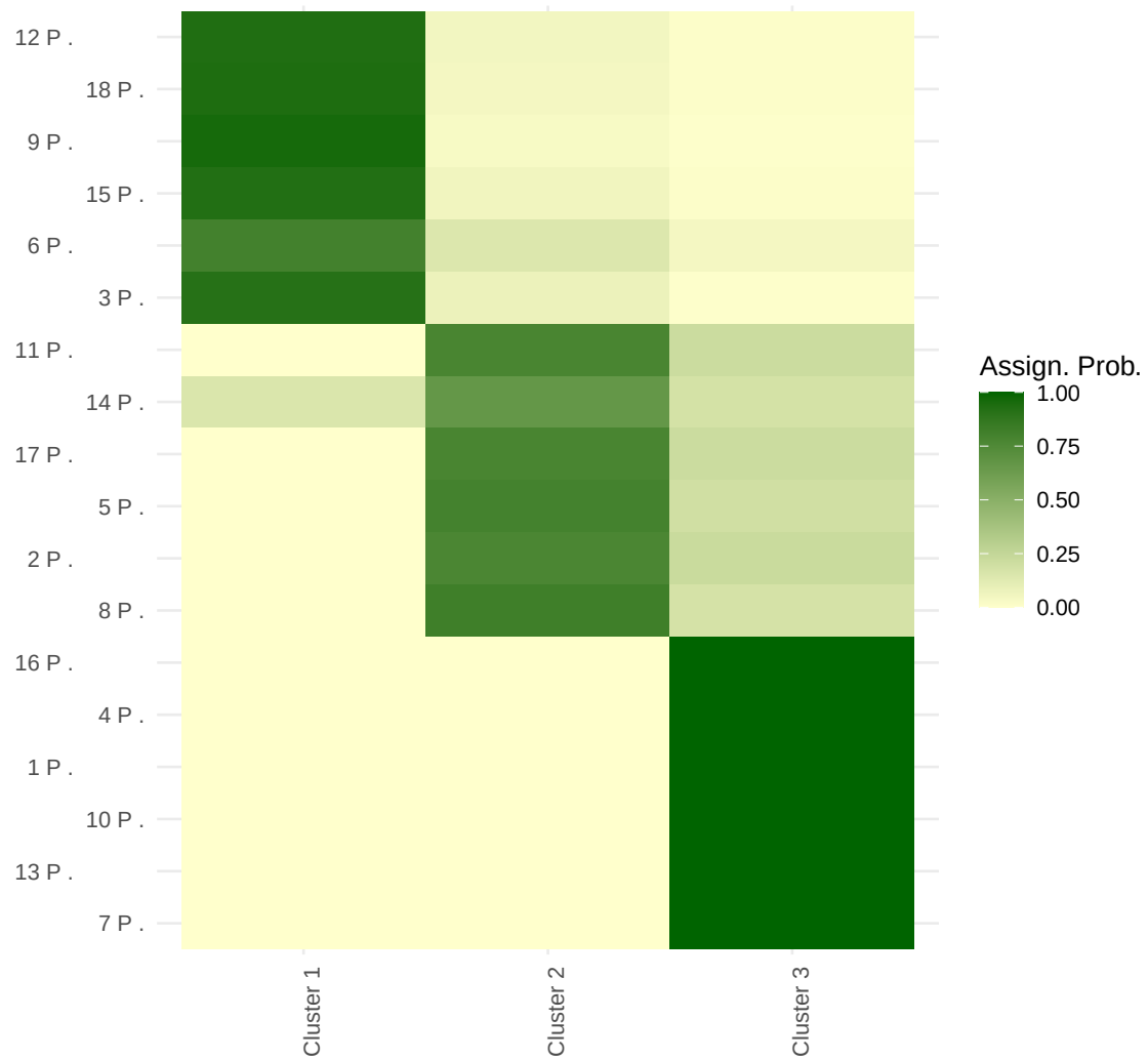
Figure 3: Posterior assignment probabilities by player and cluster, after relabelling for interpretability.
