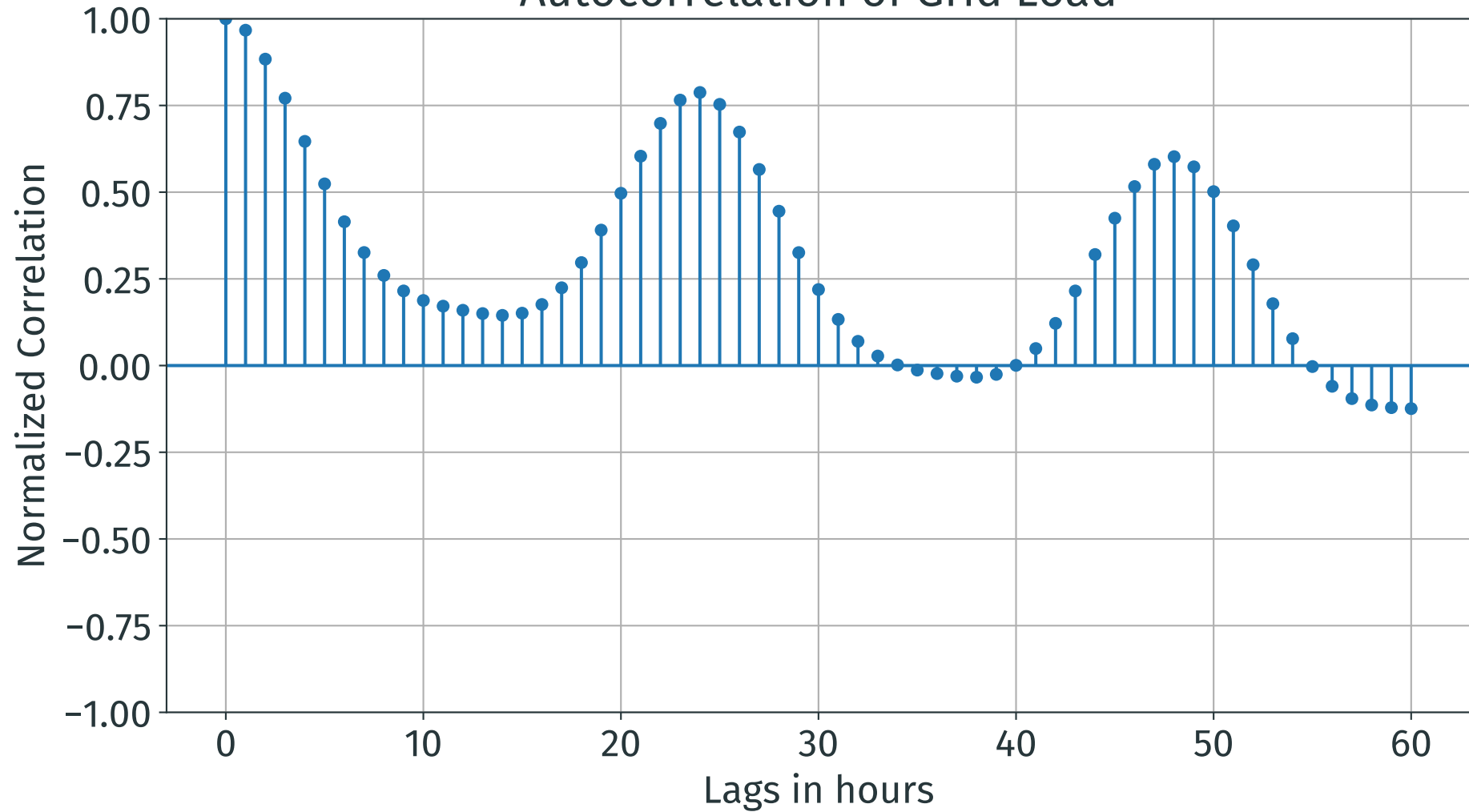
Autocorrelation of Grid Load
