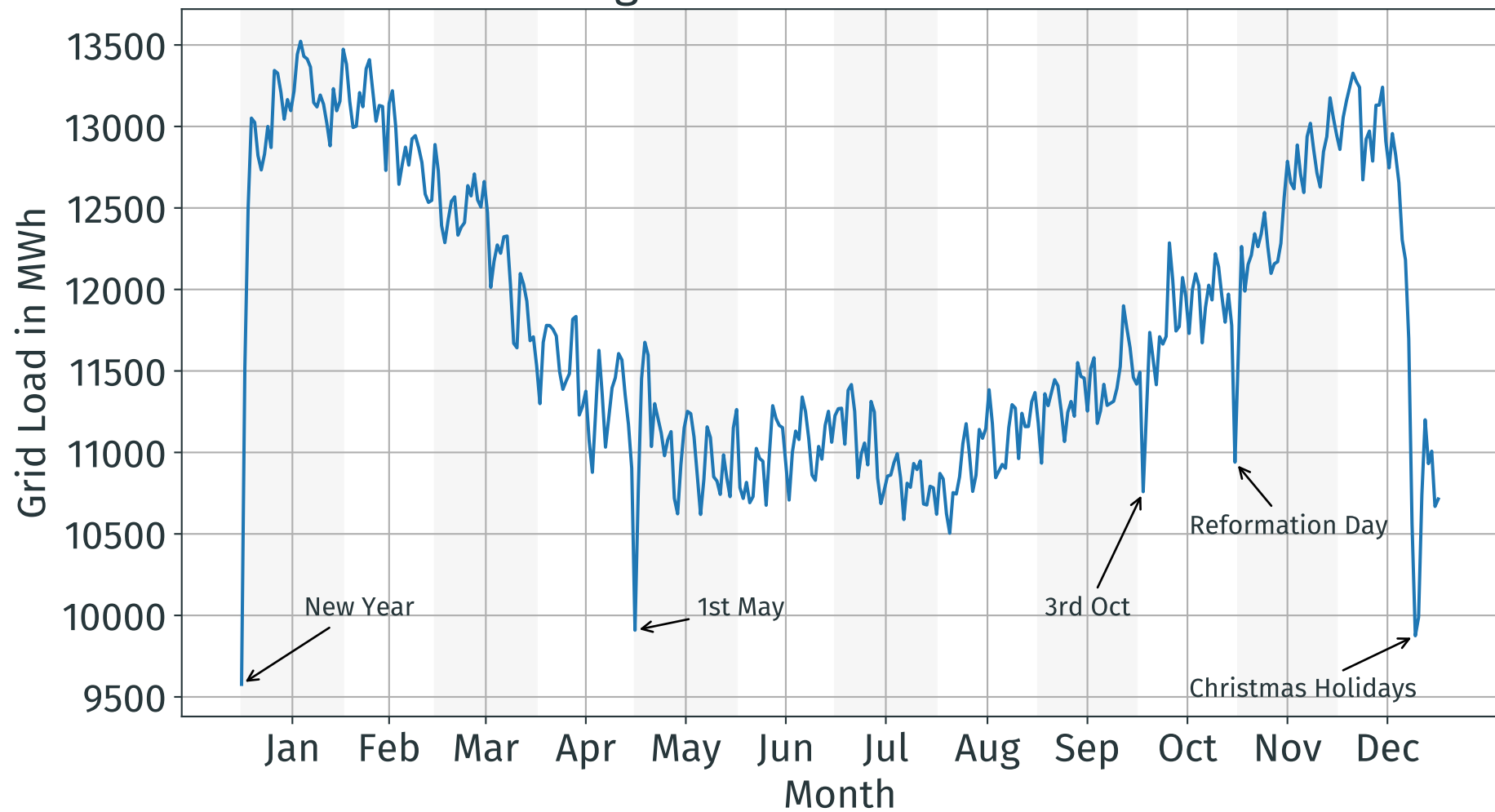
Average Grid Load Over the Year
