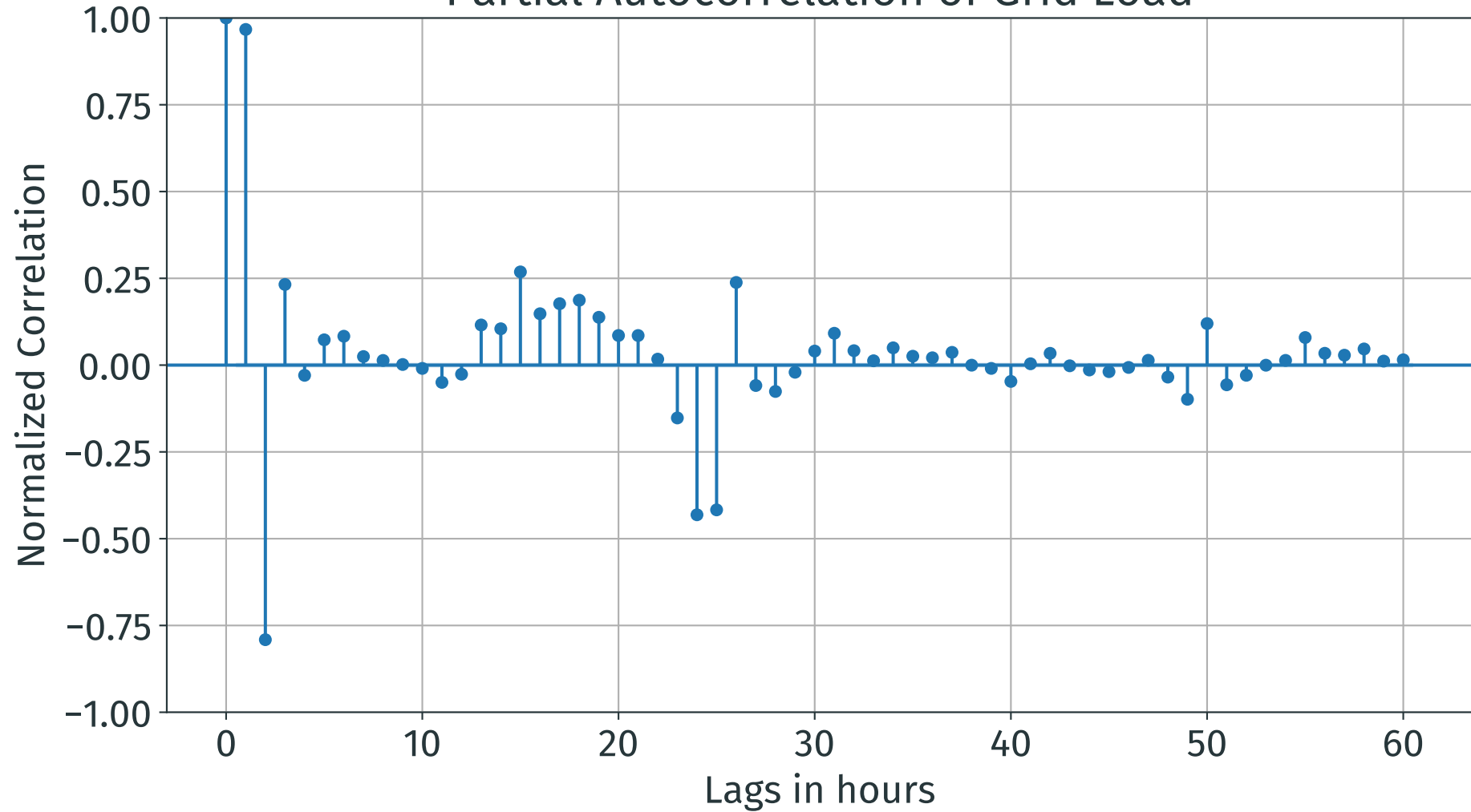
Partial Autocorrelation of Grid Load
