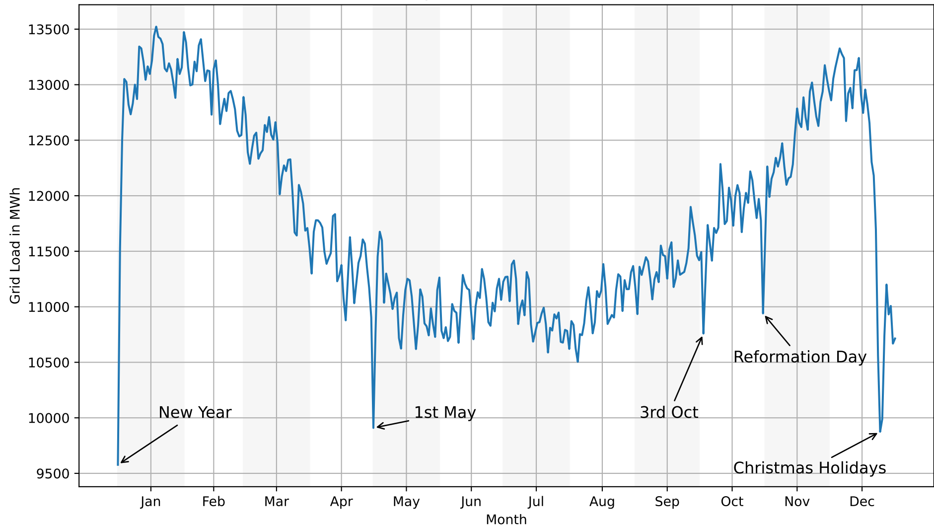
Average Grid Load Over the Year
