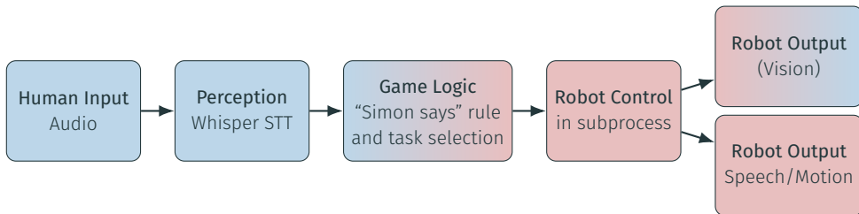
Figure 2: Processing pipeline of the Simon Says game.
