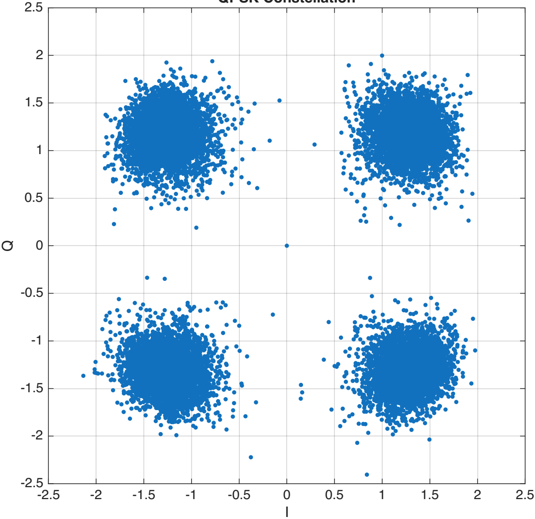
QPSK Constellation
