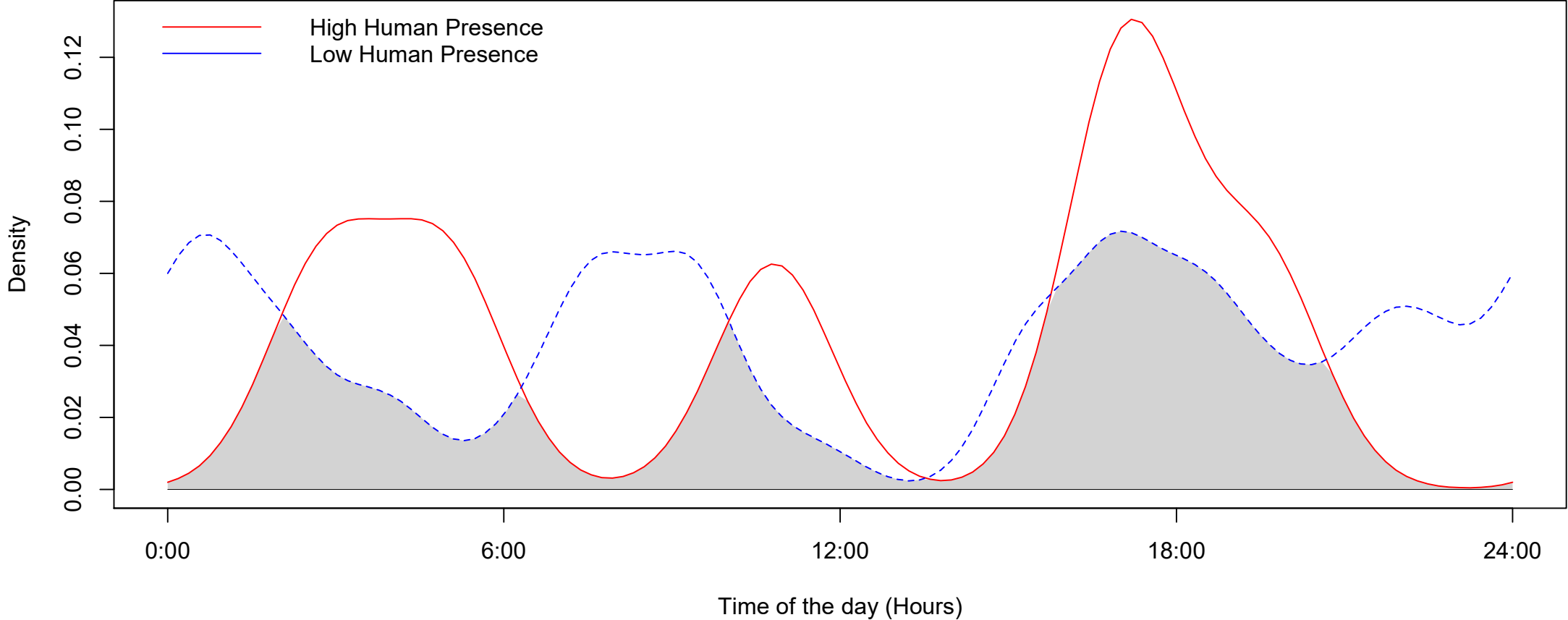
Comparison Roe Deer Activity: High vs Low Human Impact
