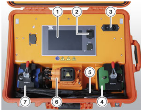
EoS tester
