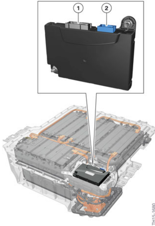
F30 PHEV battery management electronics installation location
