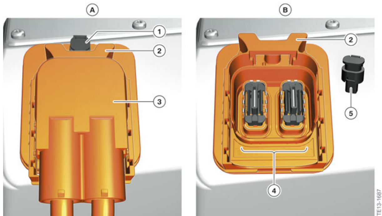
High-voltage connection
