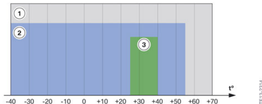
F30 PHEV high-voltage battery unit operating temperature range
