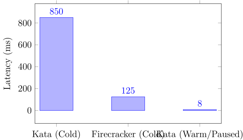
Figure 4.1: Comparison of Invocation Latency
