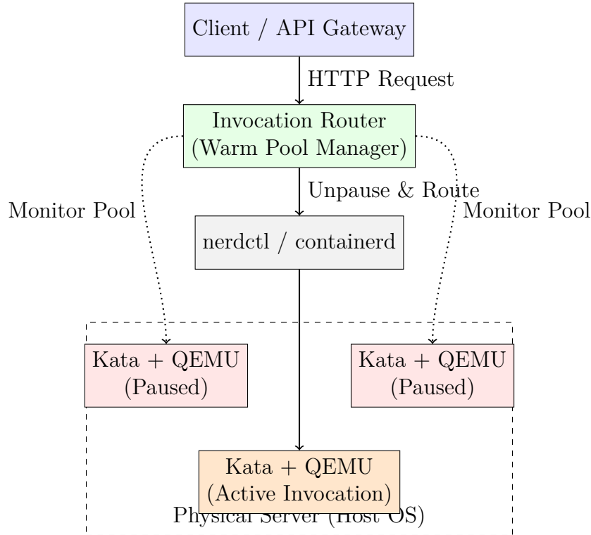
Figure 3.1: High-Level Architecture of the Warm-MicroVM Serverless Platform
