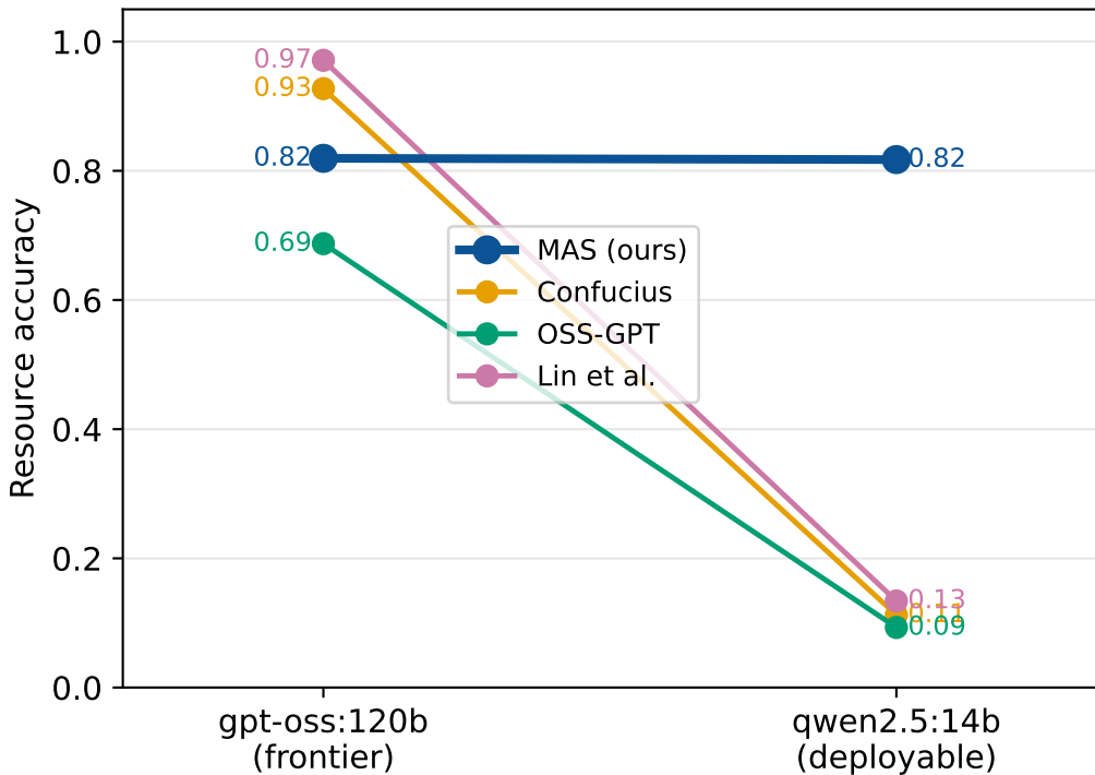
Baselines collapse on the deployable model; MAS holds
