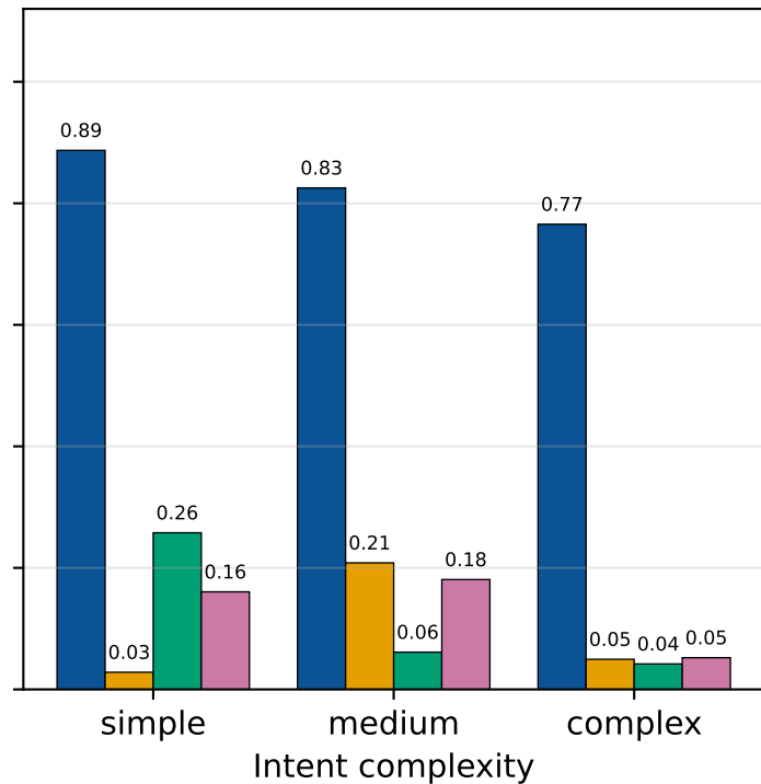
qwen2.5:14b
