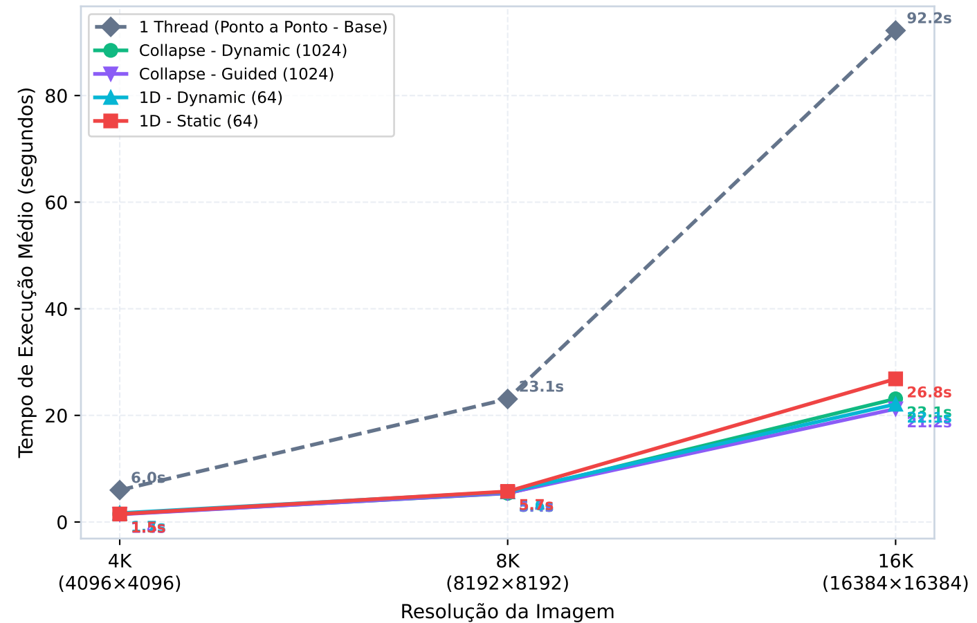
Zoom - Seahorse (Max Iter: 5000)
