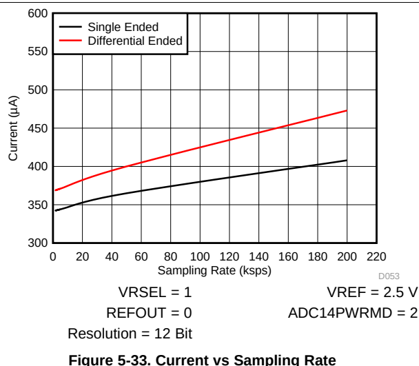
Figure 5-33. Current vs Sampling Rate
