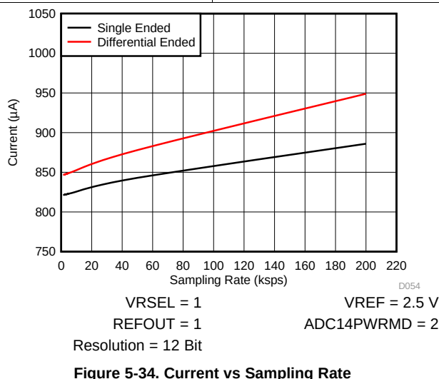
Figure 5-34. Current vs Sampling Rate
