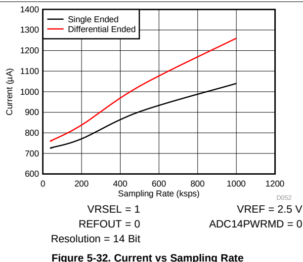
Figure 5-32. Current vs Sampling Rate
