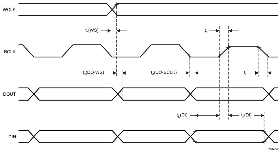
Figure 4-1. I²S/LJF/RJF Timing in Master Mode
