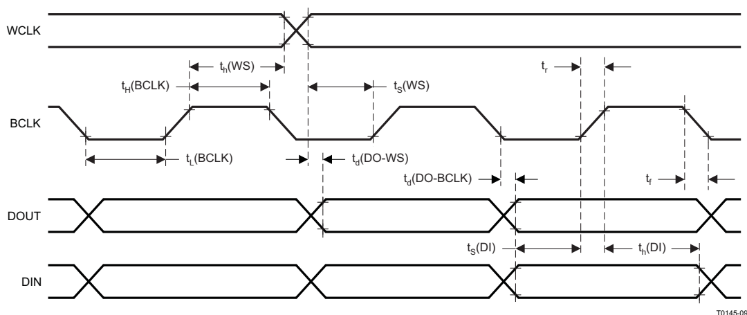
Figure 4-2. I²S/LJF/RJF Timing in Slave Mode
