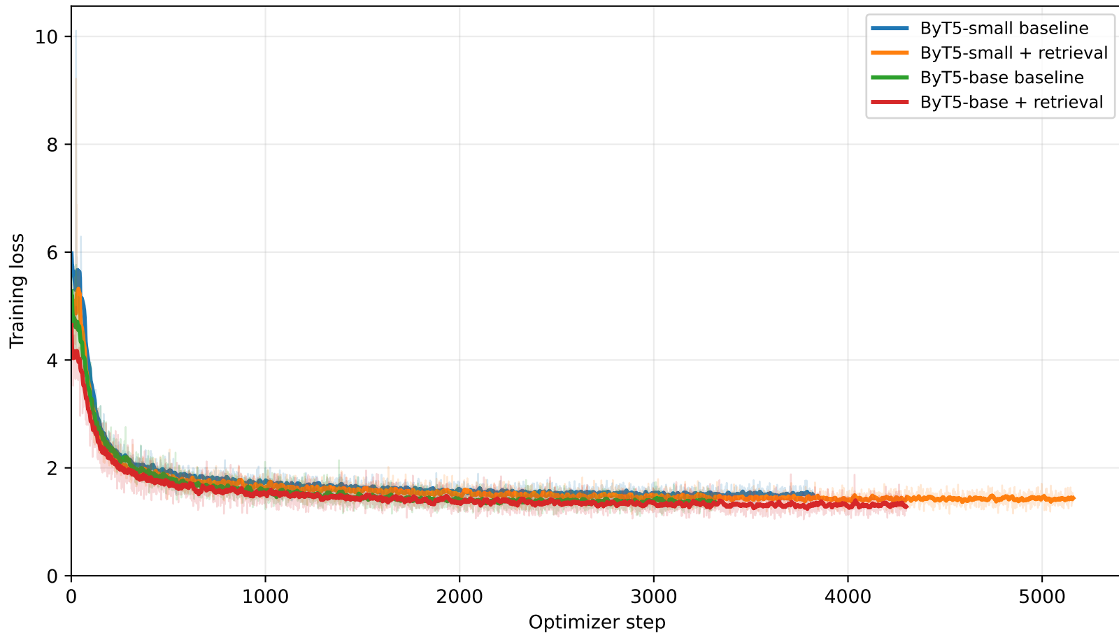
Full Retrieval vs Baseline Loss Curves
