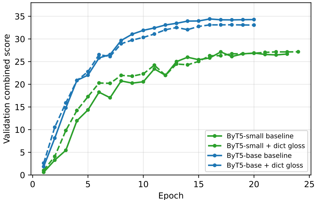
Dictionary Gloss Intervention: Validation Curves
