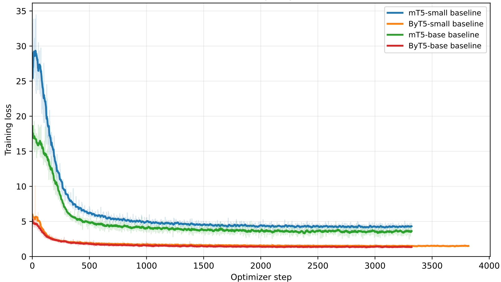
Tokenisation and Capacity Loss Curves
