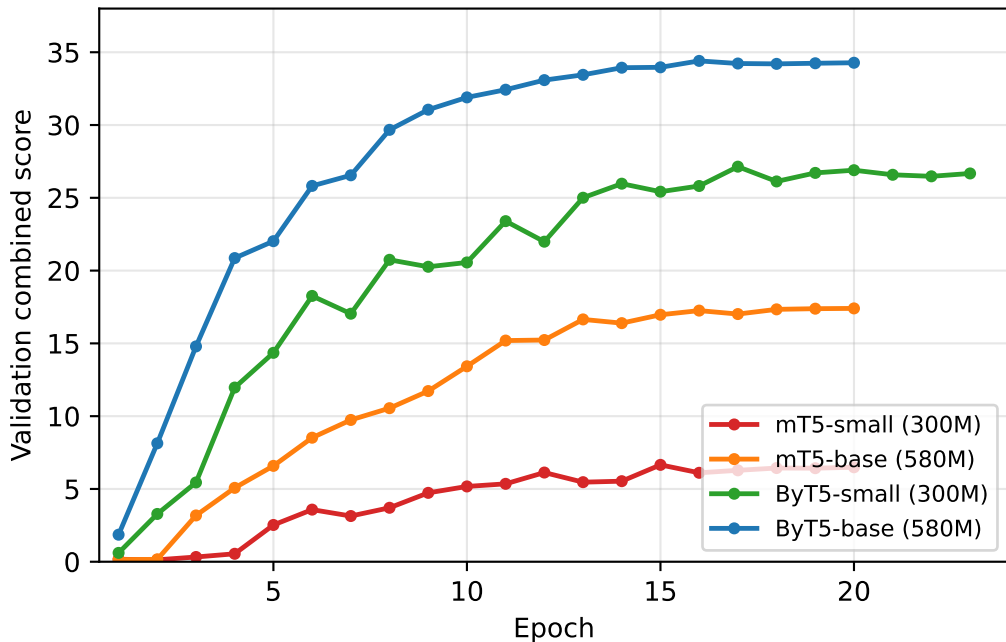
Tokenisation and Capacity: Validation Curves
