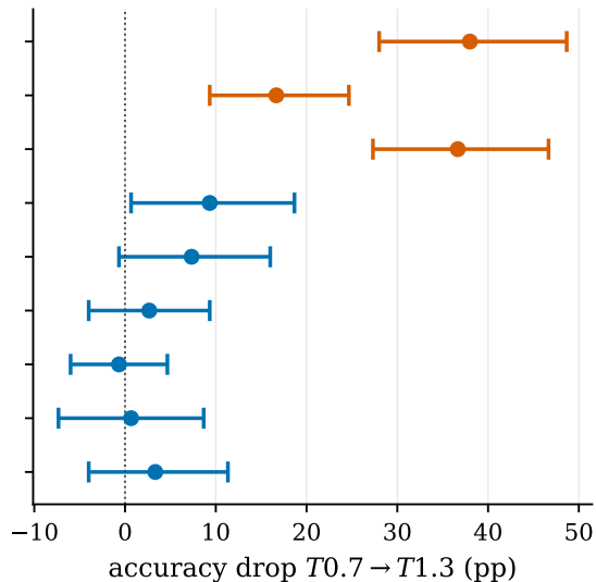
MMLU-Pro
