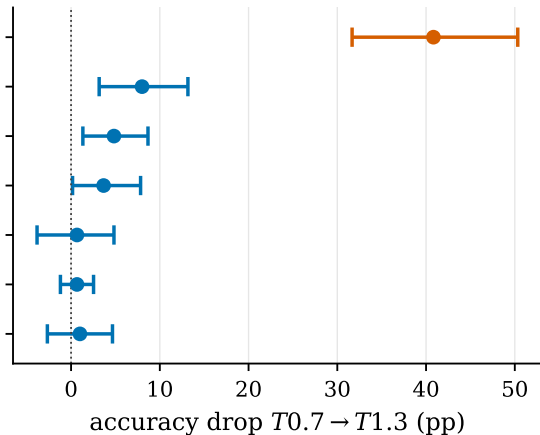
MMLU-Pro
